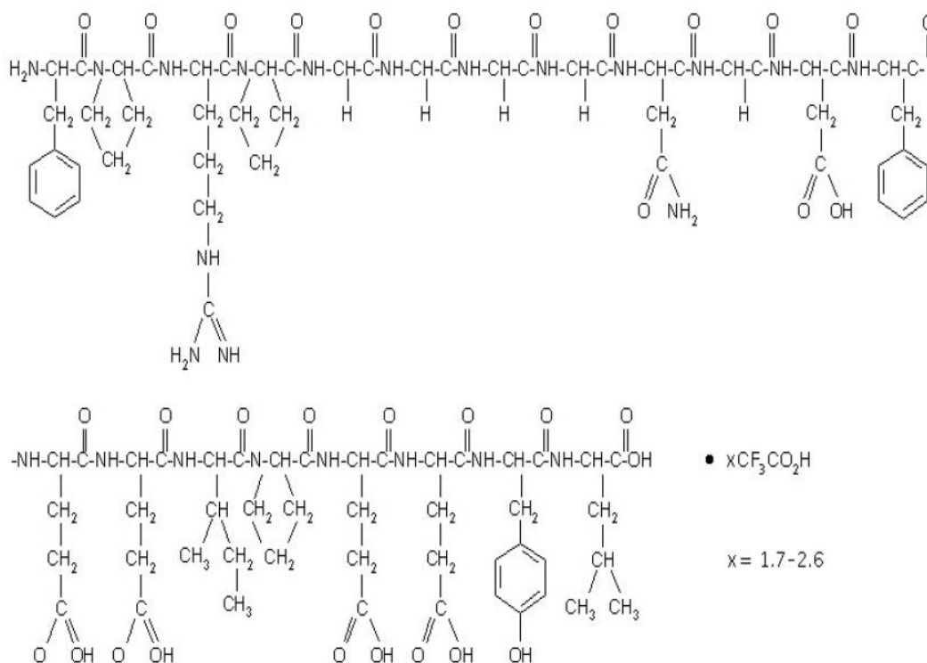
Figure 1. Structural formula for Bivalirudin trifluoroacetate
